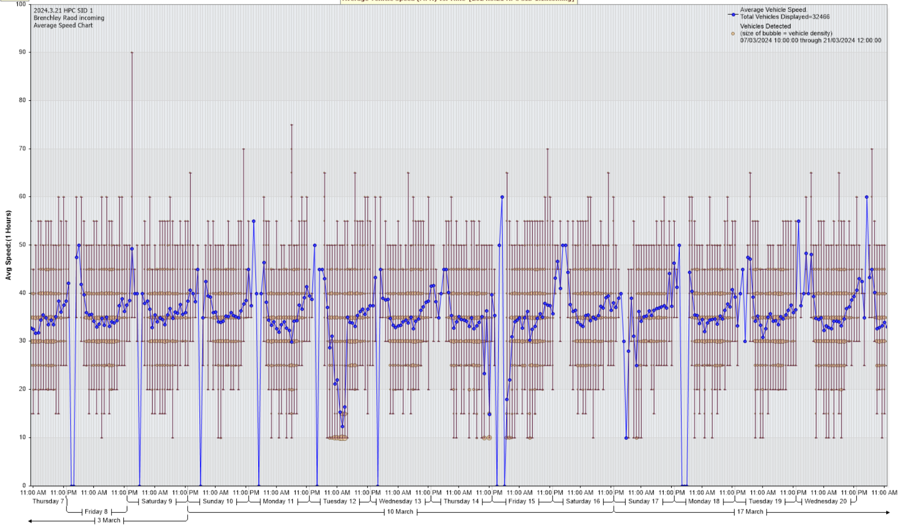
Average Vehicle Speed (MPH) vs. Time [2024.3.21 HPC SID 1:Incoming]
